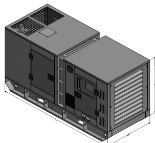
AQGT ENCLOSURE/CANOPY
